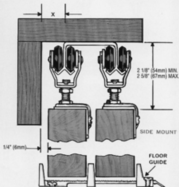
TYPICAL END VIEW DETAIL — Scale 1/2" = 1" (12.5mm = 25mm)
